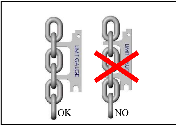
Illustration (1) Chain pitch measure
