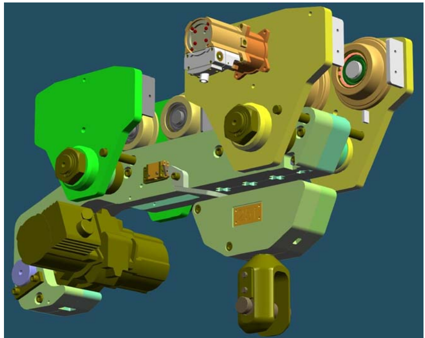
CAD model of the new JDN Low Headroom Trolley LMF 25 t
